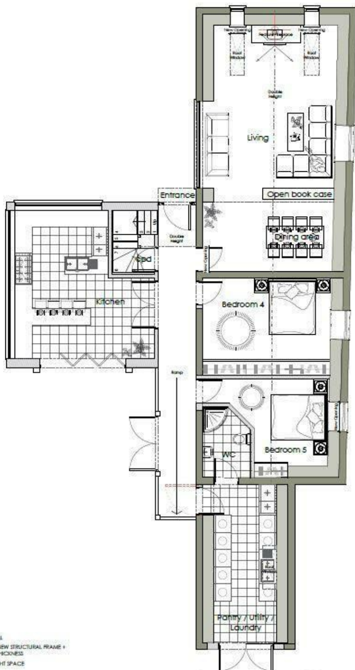
GROUND FLOOR Plan Scale 1:50
